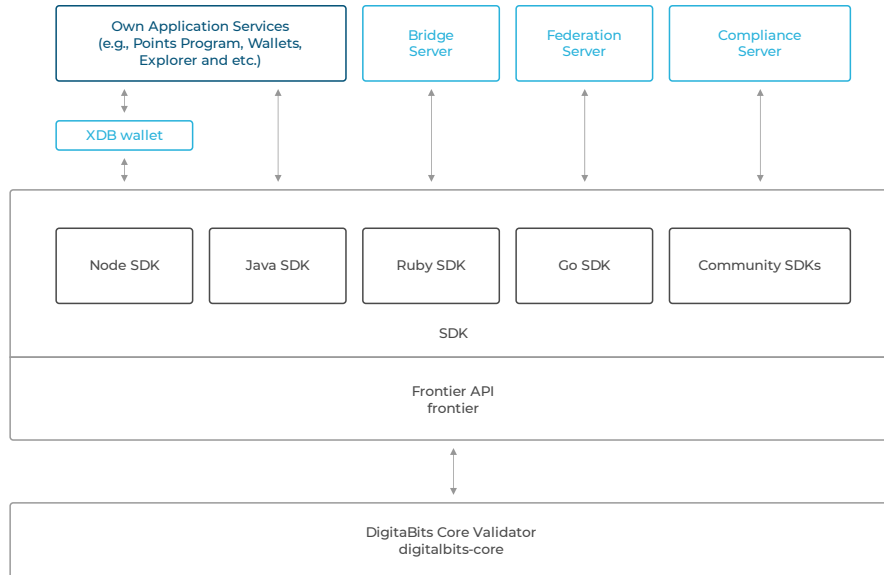
Fig. 11: Technology Stack
